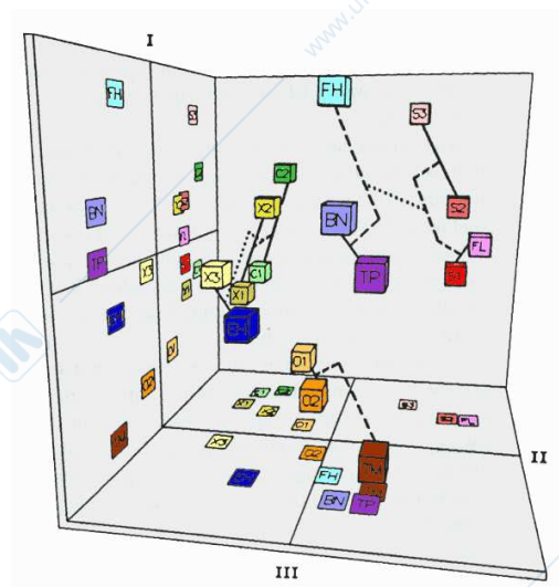
Figura 2.33: Rappresentazione dimensionale del timbro [Grey 1975]. Strumenti rappresentati: BN - Bassoon C1 - E flat Clarinet C2 - B flat Bass Clarinet EH - English Horn FH - French Horn FL - Flute O1 - Oboe O2 - Oboe (different instrument and player) S1 - Cello, muted sul ponticello S2 - Cello S3 - Cello, muted sul tasto TM - Muted Trombone TP - B flat Trumpet X1 - Saxophone, played mf X2 - Saxophone, played p X3 - Soprano Saxophone. Dimension I: spectral energy distribution, from broad to narrow. Dimension II: timing of the attack and decay, synchronous to asynchronous. Dimension III: amount of inharmonic sound in the attack, from high to none.
