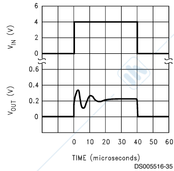
Start-Up Response
