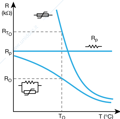
Figure 2 – Linearization of a thermistor
