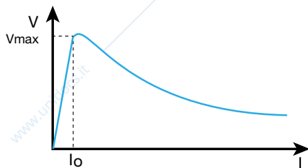
Figure 4 – Voltage – current curve V (I)
