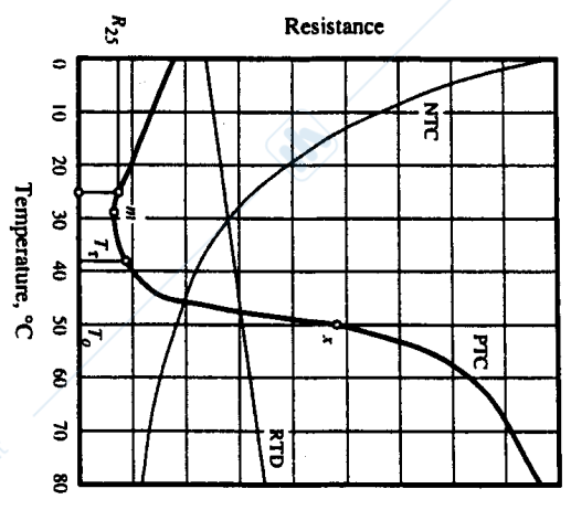
FIGURE 16.10. Transfer functions of PTC and NTC thermistors as compared with RTD.
