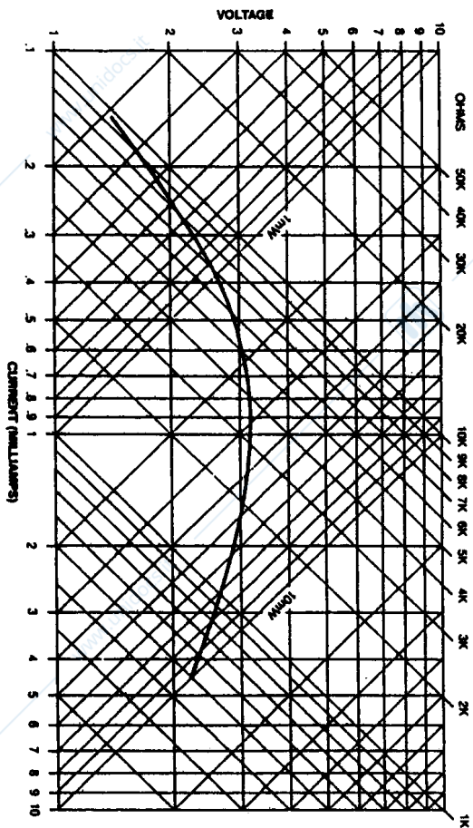
FIGURE 16.9. Voltage-current characteristic of an NTC thermistor in still air at 25 °C. (Courtesy of Thermometrics, Inc.)
