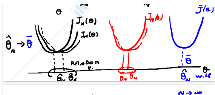
Figure 6.2: The set of minimum points for \theta_N for three increasing values of N . The right-most one is for N \rightarrow \infty .
