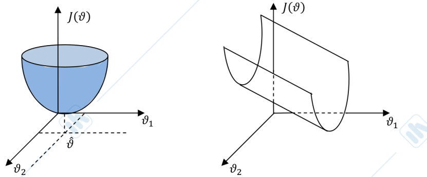
Figure 6.1: Possible shapes of J(\theta) : on the left-hand side if the matrix is positive definite, on the right-hand side if the matrix is positive semi-definite but not positive definite
